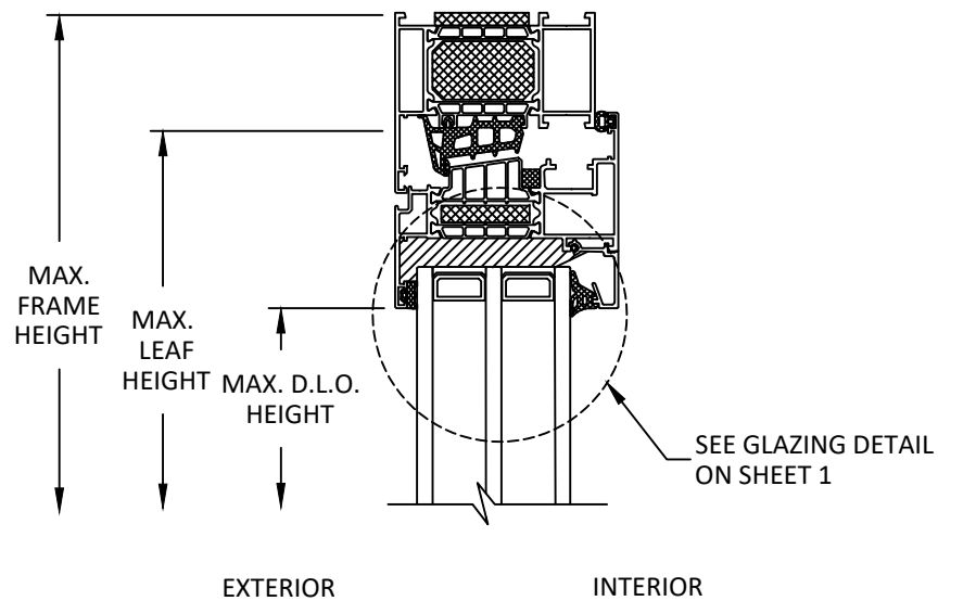
A 4 VERTICAL SECTION TYP. HEAD DETAIL
