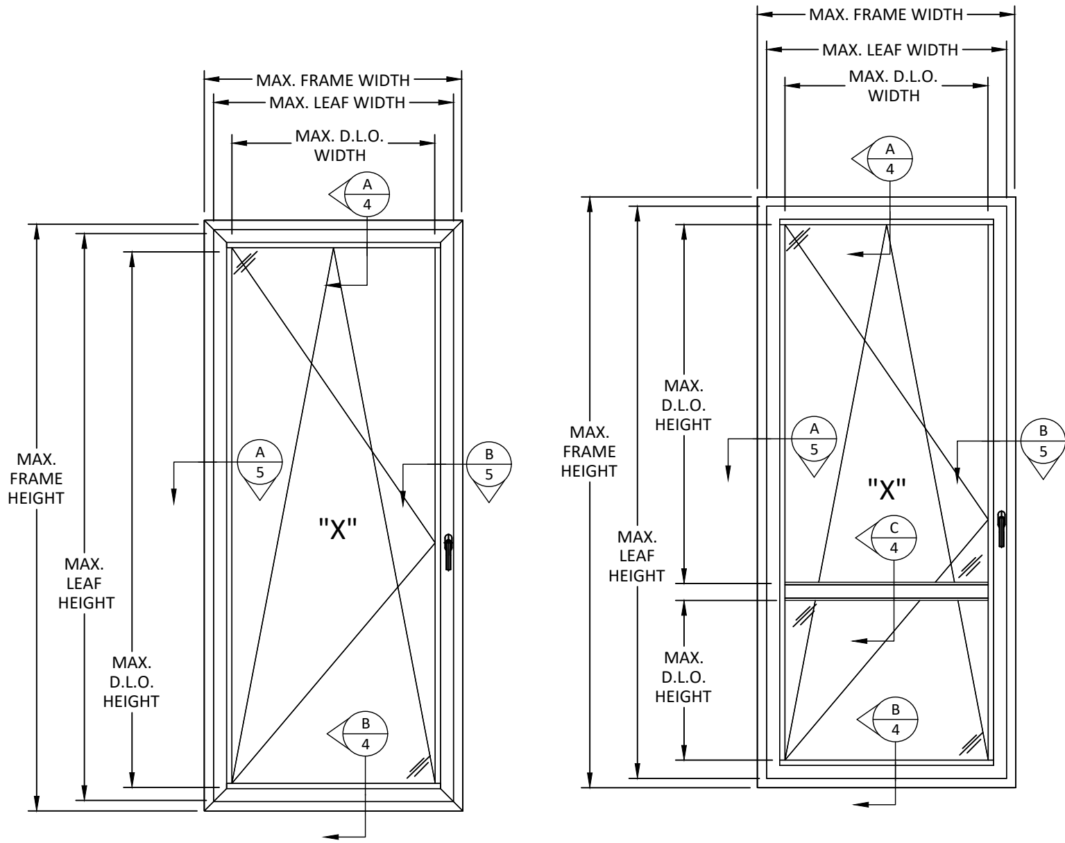
ELEVATIONS
